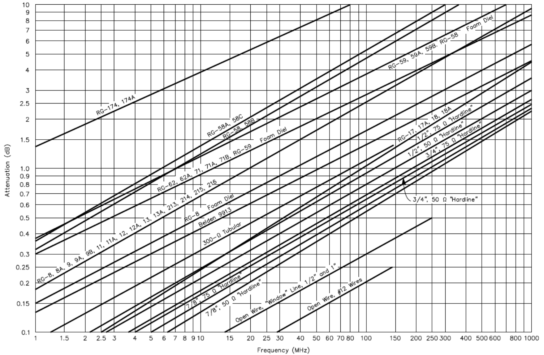
Cable Attenuation, dB Per Hundred Feet
